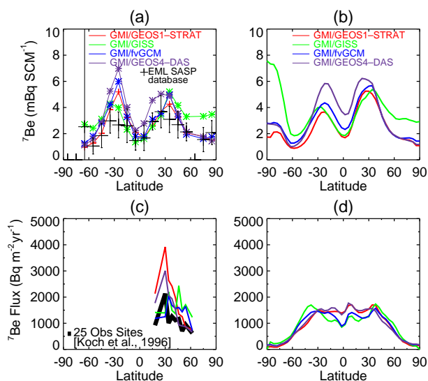
Figure 8. Same as Fig. 5, except that ^7\text{Be} cross-tropopause fluxes have been adjusted for GMI/GEOS1-STRAT and GMI/ISS.
