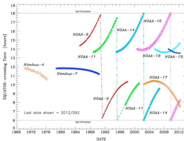
Figure 2. The local time at which each instrument in the time series crosses the equator each orbit varies due to orbit drift.
